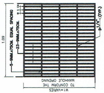
STEEL GRATING COVER DETAILS
